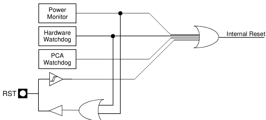
Figure 9. Reset schematic
